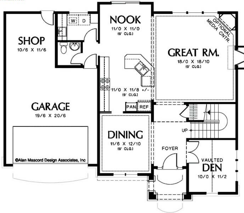
W-22151A Main Floor
