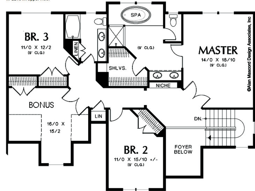
W-22151A Upper Floor
